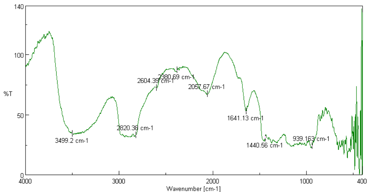
Fig 7 IR spectrum of HPMC
